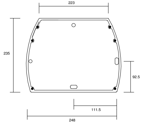
Diagram 2: Fixing details
