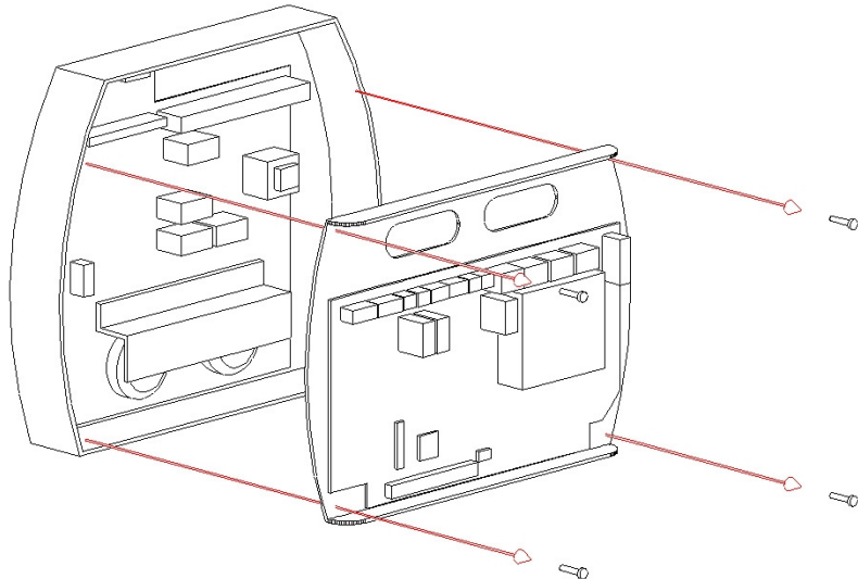
Diagram 1: Opening the unit
